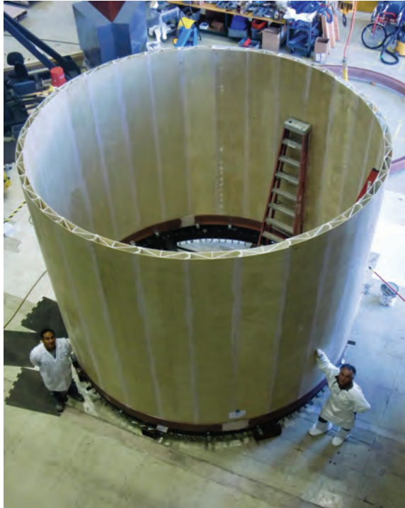
Figure 1. The first assembled core ring for 4 m diameter CWP. Note the size of the core ring compared to the two persons in the photo. Photo taken by the author.
